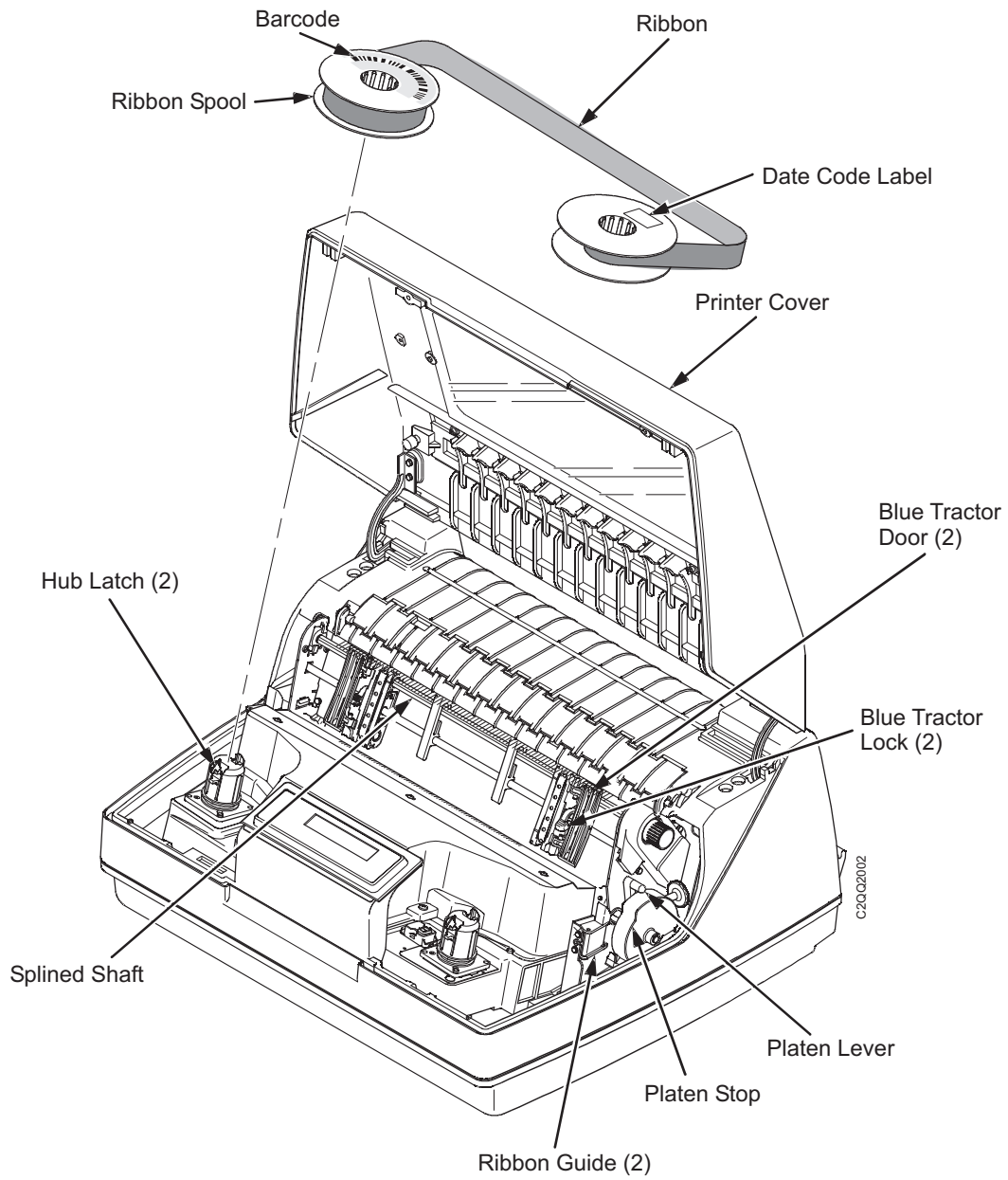
Figure 68. Interior Components of the Pedestal Models with Ribbon Spool Above
