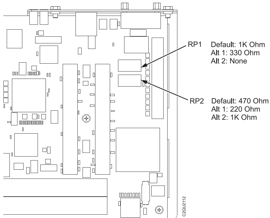
Figure 65. Resistor Locations
