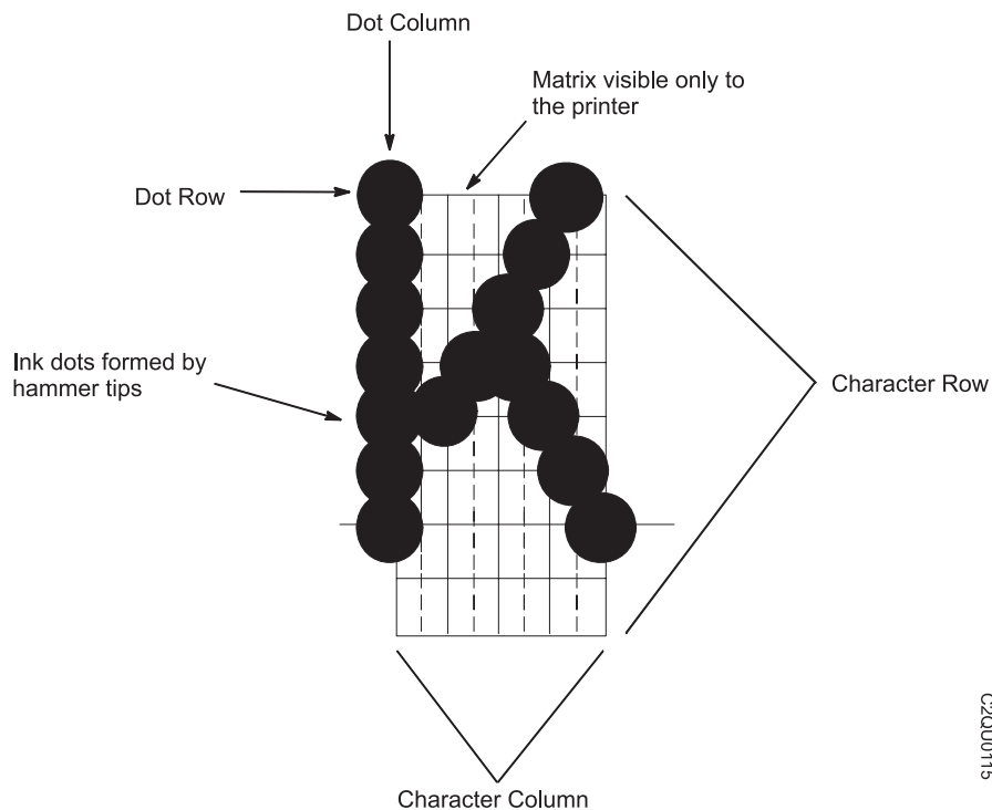
Figure 72. Typical Character Formation
