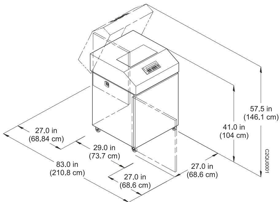
Figure 2. Exploded View of Cabinet Model Printer Dimensions
