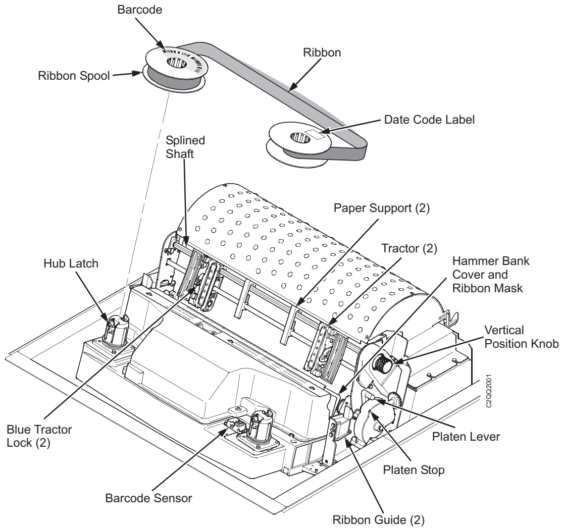
Figure 67. Interior Components of the Cabinet Models
