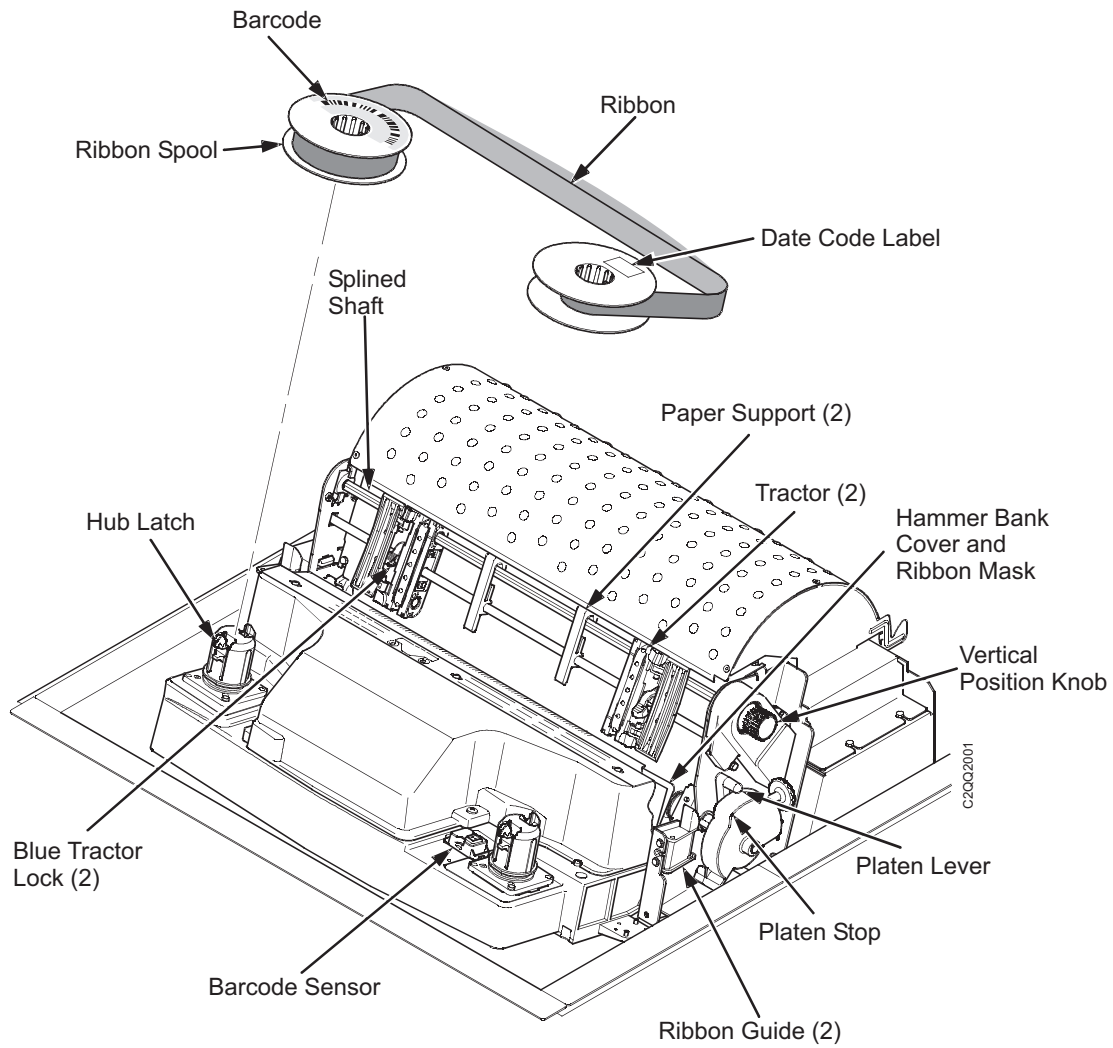
Figure 5. 6500 Printer Component Locations with the Ribbon Spools Exploded Above
